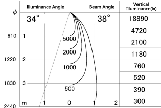
■ Direct Horizontal Illuminance SD348-2940W9030
