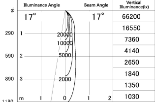
■ Direct Horizontal Illuminance SD348-2915W8030
