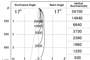
■ Direct Horizontal Illuminance SD348-2915W8527
