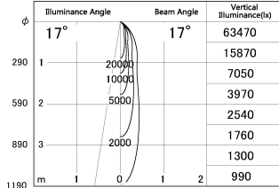
■ Direct Horizontal Illuminance SD348-2915W8535
