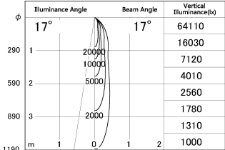
Direct Horizontal Illuminance SD348-2915W8540
