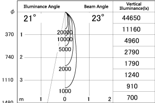
Direct Horizontal Illuminance SD348-2920W8035
