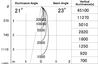
Direct Horizontal Illuminance SD348-2920W8040
