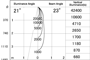
Direct Horizontal Illuminance SD348-2920W8540
