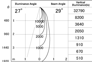
■ Direct Horizontal Illuminance SD348-2930W8040
