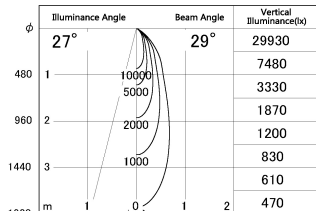
■ Direct Horizontal Illuminance SD348-2930W8530
