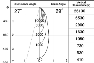
Direct Horizontal Illuminance SD348-2930W9027
