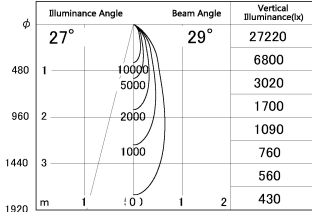
■ Direct Horizontal Illuminance SD348-2930W9030
