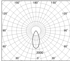
Lighting Distribution Curve (cd./1000 m)
