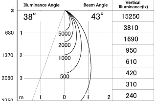
Direct Horizontal Illuminance SD348-3040W9035
