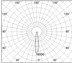
■ Lighting Distribution Curve (cd./1000 m)
