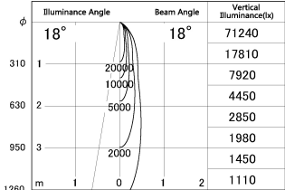
■ Direct Horizontal Illuminance SD348-3020W8027
