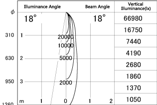
Direct Horizontal Illuminance SD348-3020W8527
