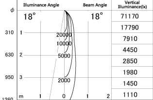
■ Direct Horizontal Illuminance SD348-3020W8535
