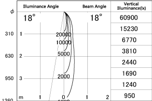
■ Direct Horizontal Illuminance SD348-3020W9027
