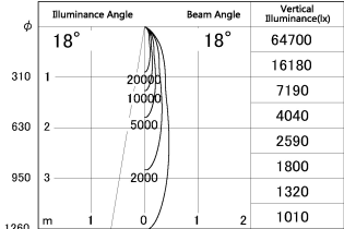
■ Direct Horizontal Illuminance SD348-3020W9035
