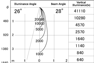
■ Direct Horizontal Illuminance SD348-3030W8030
