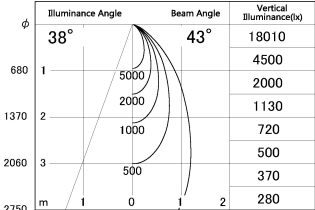
■ Direct Horizontal Illuminance SD348-3040W8040
