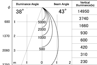
■ Direct Horizontal Illuminance SD348-3040W9030
