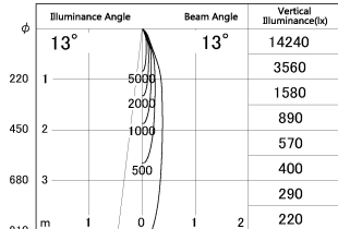
■ Direct Horizontal Illuminance DD052-0815MW9030
