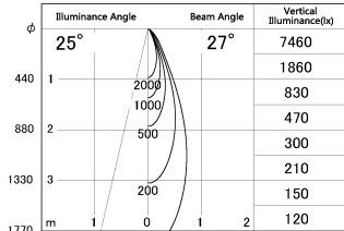
■ Direct Horizontal Illuminance DD052-0825MW9040
