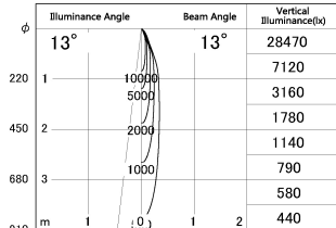
■ Direct Horizontal Illuminance DD052-1315MW9035
