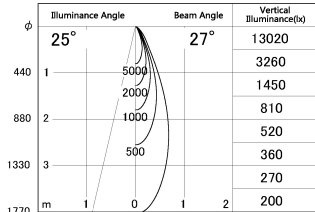
■ Direct Horizontal Illuminance DD052-1325MW9035
