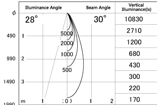
■ Direct Horizontal Illuminance DD052-1330MW9035
