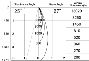
■ Direct Horizontal Illuminance DD052-1325MW9035-DM
