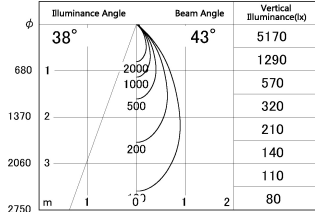
■ Direct Horizontal Illuminance DD052-1340MW9035-DM
