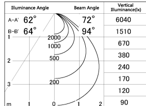
■ Direct Horizontal Illuminance SD346-36W8535
