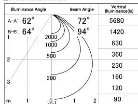
■ Direct Horizontal Illuminance SD346-36W8527
