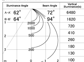
■ Direct Horizontal Illuminance SD346-36W8040
