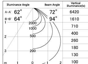
■ Direct Horizontal Illuminance SD346-36W8035
