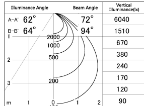
■ Direct Horizontal Illuminance SD346-36W8027
