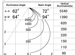
■ Direct Horizontal Illuminance SD346-36B9040
