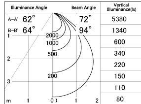
■ Direct Horizontal Illuminance SD346-36B9030
