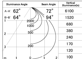
■ Direct Horizontal Illuminance SD346-36B8540
