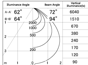
■ Direct Horizontal Illuminance SD346-36B8535
