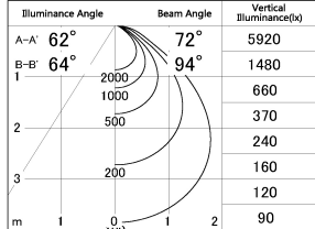
■ Direct Horizontal Illuminance SD346-36B8530
