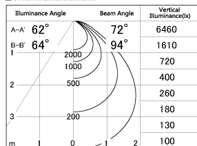
■ Direct Horizontal Illuminance SD346-42W9035
