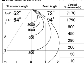
■ Direct Horizontal Illuminance SD346-42W8540
