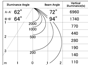
■ Direct Horizontal Illuminance SD346-42W8530
