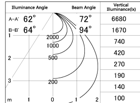
■ Direct Horizontal Illuminance SD346-42W8527
