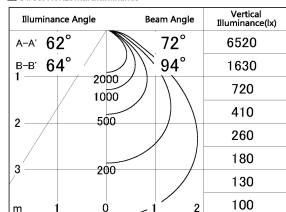
■ Direct Horizontal Illuminance SD346-42B9040
