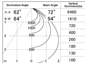
■ Direct Horizontal Illuminance SD346-42B9035
