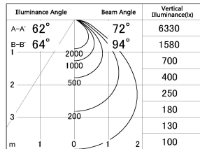
■ Direct Horizontal Illuminance SD346-42B9030
