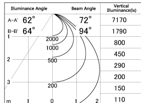
■ Direct Horizontal Illuminance SD346-42B8540
