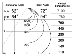
■ Direct Horizontal Illuminance SD346-42B8535
