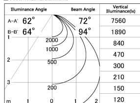
■ Direct Horizontal Illuminance SD346-42W8035
