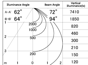
■ Direct Horizontal Illuminance SD346-42B8030
